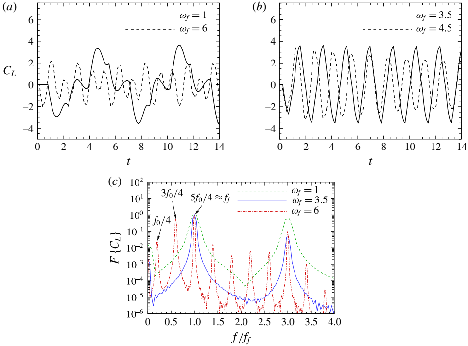
FIGURE 11. (Colour online) A typical time variation of the cylinder lift coefficient for I=12 and \omega_f as indicated within (a) unlock-in regimes and (b) lock-in regimes. (c) Respective Fourier spectra of the lift coefficient signals in (a) and (b).
