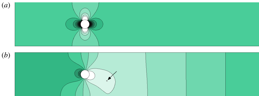
FIGURE 3. (Colour online) Contour plots of the difference in electrical potential field calculated from the analytical solution and the field that is solved numerically in the presence of the electrically insulating cylinder. In (a), current is injected from the base of the cylinder and contour levels range between -0.001 and 0.001 , and in (b), current is injected from an electrode placed at l_x = 1 and l_y = 0.7 (indicated by the arrow), and contour levels range between -0.04 and 0.06 . Light and dark contours represent positive and negative difference in electrical potential, respectively.
