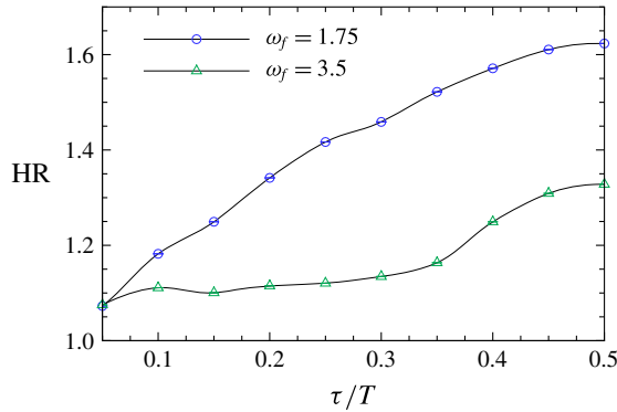
FIGURE 16. (Colour online) Heat transfer enhancement ratio plotted against current injection pulse width \tau/T at frequencies \omega_f as indicated for H=500 , I=30 and G/d=2 . The current is injected from the cylinder.
