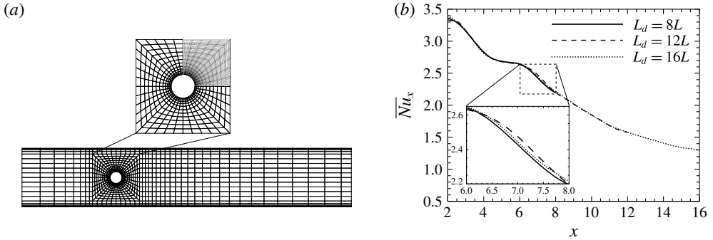
FIGURE 4. (a) Macro-element distribution of the computational domain, and magnified mesh in the vicinity of the cylinder, with the upper right quadrant representing the distribution of collocation points within elements with N_p = 8 . The mesh extends 3.2L upstream and 8L downstream. (b) Time-averaged local Nusselt number in the downstream of cylinder for H = 500 , Re_L = 1500 , I = 60 , \omega_f = 1.75 and \tau/T = 0.25 . Solid, dashed and dotted lines represent domains with respective downstream lengths L_d = 8L , 12L and 16L .
