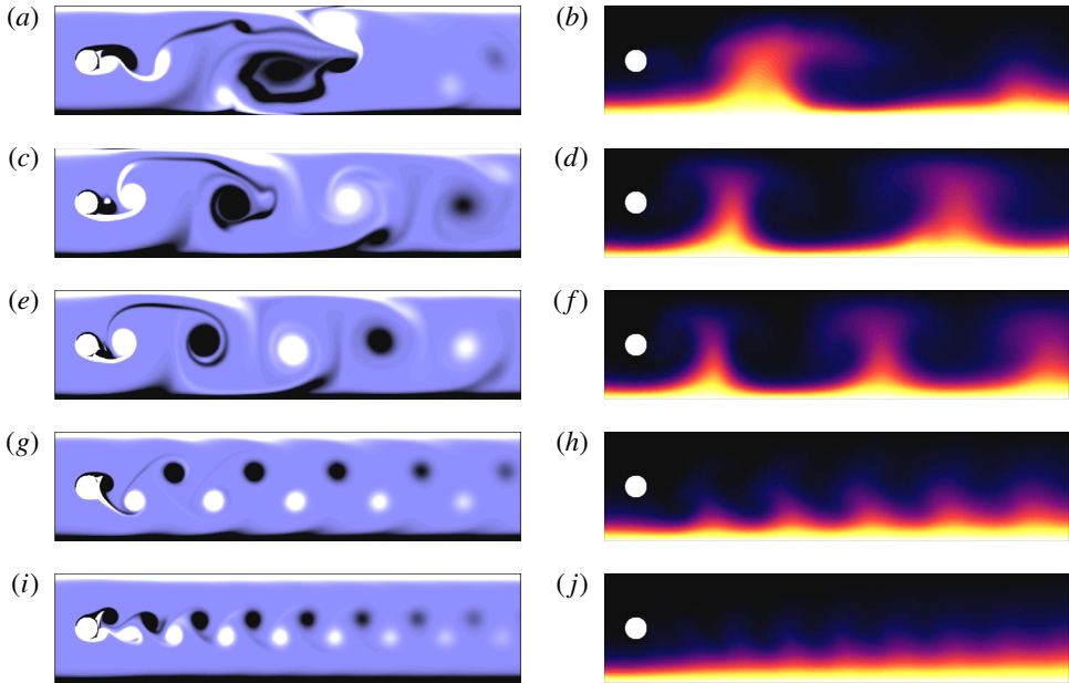
FIGURE 7. (Colour online) Contour plots of vorticity ( a,c,e,g,i ) and temperature ( b,d,f,h,j ) for current injection amplitude I=30 and forcing frequencies 0.5 \leq \omega_f \leq 6 . Vorticity fields: contour levels are as per figure 5. Temperature fields: dark and light contours show cold and hot fluid, respectively. ( a,b ) \omega_f = 0.5 , ( c,d ) 1.5, ( e,f ) 2, ( g,h ) 4, ( i,j ) 6.
