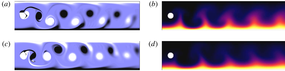
FIGURE 9. (Colour online) Instantaneous vorticity and temperature contour plots for I = 60 and (a,b) \omega_f = 3.375 and (c,d) \omega_f = 3.3125 . Contour levels are as per figure 5. (a,c) Vorticity fields, (b,d) temperature fields.
