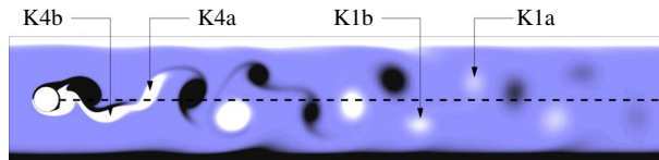
FIGURE 8. (Colour online) Instantaneous vorticity contour plots for I=12 and \omega_f=6 . The dashed line represents the duct centreline. Contour levels ranges between -1 and 1 , with light and dark contours represent positive and negative vorticity, respectively.
