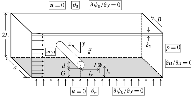
FIGURE 1. Schematic diagram of the system under investigation. The cylinder spans the duct, with diameter d and axis parallel to z -direction, and the small circle indicates a point electrode embedded in one of the Hartmann walls.
