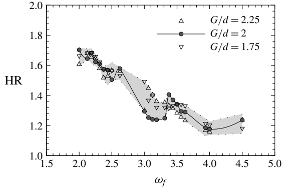
FIGURE 10. Time-averaged heat transfer enhancement plotted against forcing frequency for I = 60 , \tau/T = 0.25 , and \omega_f and G/d as indicated. The current is injected from the cylinder. The shaded region highlights the zone bounded by \max(\text{HR} + \sigma_{HR}) and \min(\text{HR} - \sigma_{HR}) , where \sigma_{HR} is the standard deviation of mean HR.
