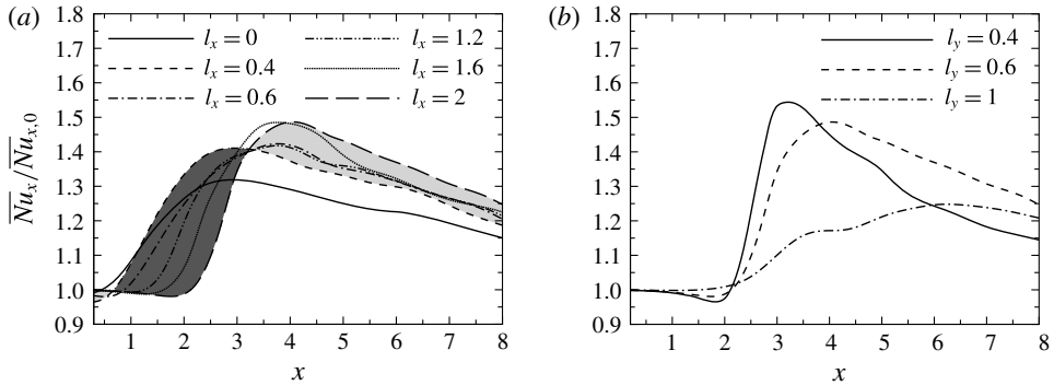
FIGURE 19. Normalized time-averaged local Nusselt number along the downstream of the heated wall. (a) The electrode is placed at l_y = 0.6 and at l_x as indicated. The dark (lighter) region correspond to a deficit (surplus) in heat transfer enhancement of case with l_x = 2 relative to the case with l_x = 0.4 . (b) The electrode is placed at l_x = 2 and at l_y as indicated.
