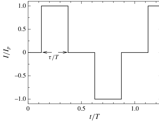
FIGURE 2. Typical electric current injection profile, represented by a modified square waveform with pulse width 0 < \tau/T < 0.5 . In the limit of \tau/T = 0.5 , the current injection profile takes a square waveform. The amplitude of current is normalized by its peak amplitude, I_p , and the time is normalized by signal period, T .
