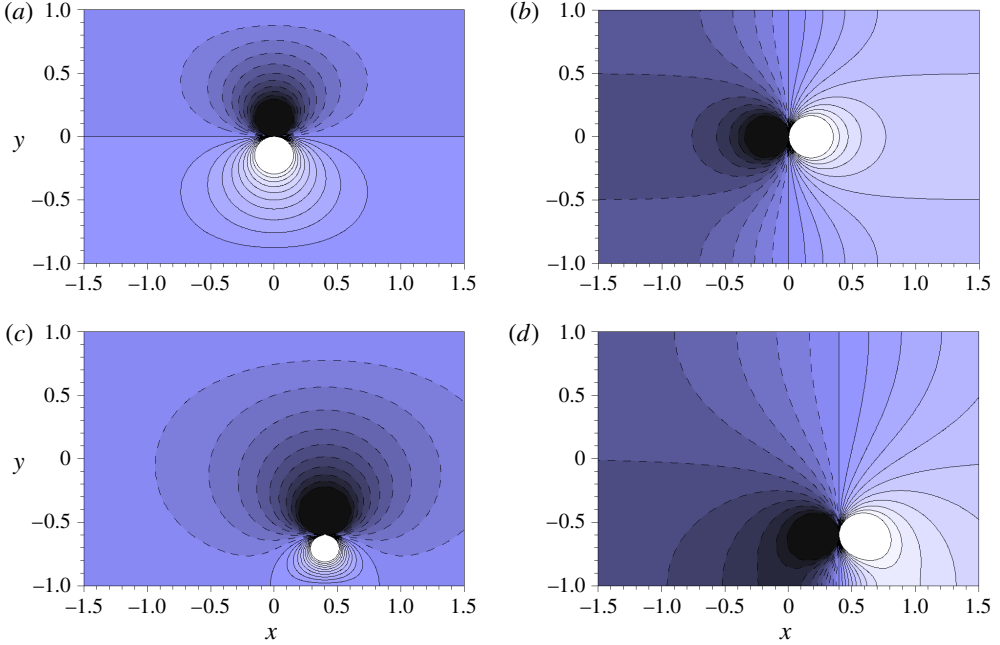
FIGURE 23. (Colour online) Contour plots of the horizontal ( a,c ) and vertical ( b,d ) components of \mathbf{u}_0 for I = 60 , H = 500 , Re_L = 1500 and electrode locations ( a,b ) (x, y) = (0, 0) and ( c,d ) (x, y) = (0.4, -0.6) . Contour levels range between -5 and 5 , with light and dark contours representing positive and negative velocity, respectively.
