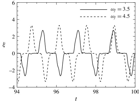
FIGURE 12. Time history of vorticity signal taken at (x, y) = (0, 5d) for I = 12 and \omega_f as indicated.
