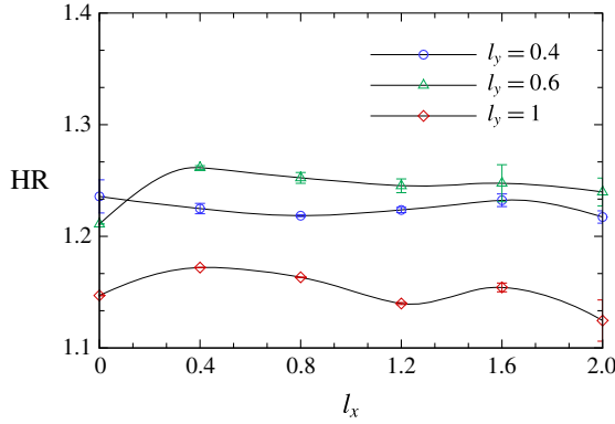
FIGURE 18. (Colour online) Heat transfer enhancement ratio plotted against horizontal distance l_x at vertical distance l_y as indicated for I = 12 , \omega_f = 1.75 , \tau/T = 0.25 and G/d = 2 .
