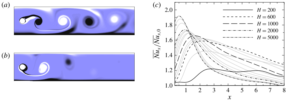
FIGURE 21. (Colour online) (a, b) Instantaneous vorticity contour plots for Re_L = 1500 and (a) H = 300 and (b) H = 1500 . Contour levels are as per figure 5. (c) Normalized time-averaged local Nusselt number along the downstream of the heated wall for Re_L = 1500 and H as indicated.
