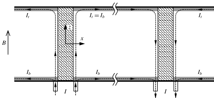
FIGURE 24. Schematic representation of the electric current paths (dotted lines) from a ring of electrodes around the base of the cylinder (the cylinder is represented by a diagonal line shading) in the limit of high Hartmann number and interaction parameter. The electrode is embedded into one of the Hartmann walls and made flush with the surface to avoid disturbance of the flow. The Hartmann layers are shaded grey, which contain most of the current paths in for quasi-2-D flow.
