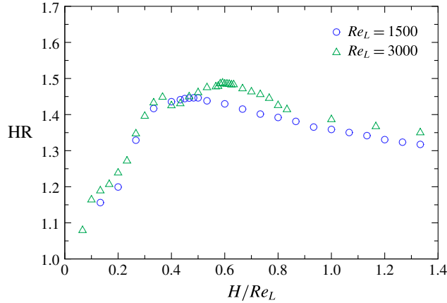
FIGURE 22. (Colour online) Heat transfer enhancement ratio and plotted against H/Re_L for Re_L as indicated. Circle and delta symbols represent Re_L = 1500 and 3000 , respectively.
