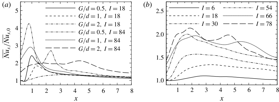
FIGURE 14. Normalized time-averaged local Nusselt number along the downstream of the heated wall for \tau/T = 0.25 , \omega_f = 1.75 and (a) I and G/d as indicated, and (b) G/d = 2 and I as indicated.
