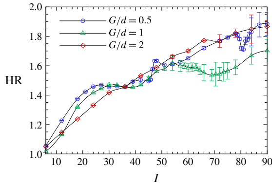
FIGURE 13. (Colour online) Heat transfer enhancement ratio plotted against current injection amplitude I at gap ratios G/d as indicated for H = 500 , \tau/T = 0.25 and \omega_f = 1.75 . The current is injected from the cylinder.
