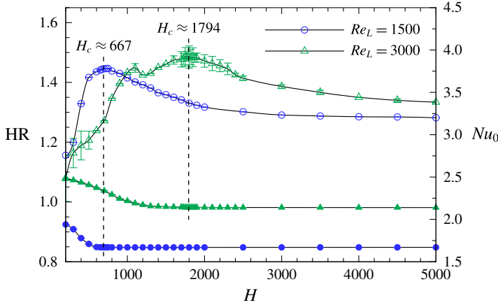
FIGURE 20. (Colour online) (Primary vertical axis) heat transfer enhancement ratio and (secondary vertical axis) base flows time-averaged Nusselt number plotted against friction parameter H for Reynolds numbers Re_L = 1500 and 3000 . Open symbols represent HR and solid symbols represent Nu_0 . The dashed lines indicate a critical value of the friction parameter, above which the cylinder vortex shedding is completely suppressed.
