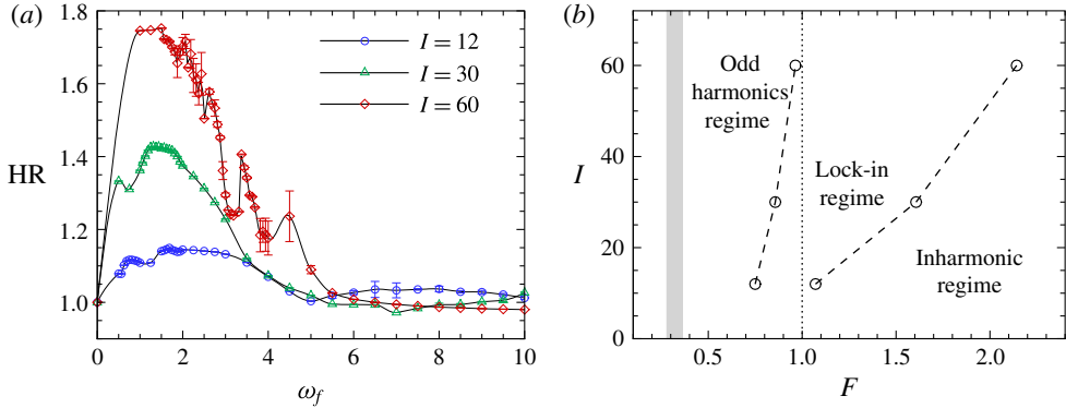
FIGURE 6. (Colour online) (a) Time-averaged heat transfer enhancement plotted against forcing frequency \omega_f at non-dimensional current amplitudes I as indicated for \tau/T = 0.25 and G/d = 2 . The current is injected from the cylinder. Error bars represent standard deviations of the mean Nusselt number within a shedding cycle evaluated at various shedding phases. (b) Limits of the lock-in regime as a function of forcing amplitude and normalized forcing frequency F = f_f/f_0 . Regime to the left (right) of the lower (upper) bound represent wakes with odd harmonics (inharmonic) in cylinder lift force. The dotted line represent F = f_f/f_0 = 1 , and the shaded region highlights the zone where HR is maximum.
