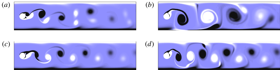
FIGURE 17. (Colour online) Instantaneous vorticity contour plots for I=30 and (a) \omega_f = 1.75 and (b) \omega_f = 3.5 . Contour levels are as per figure 5. (a,c) \tau/T = 0.05 , (b,d) 0.5.
