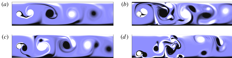
FIGURE 15. (Colour online) Instantaneous vorticity contour plots for (a) I = 30 and G/d = 2 , (c) I = 54 and G/d = 2 , (b) I = 78 and G/d = 2 and (d) I = 84 and G/d = 0.5 . Contour levels are as per figure 5.
