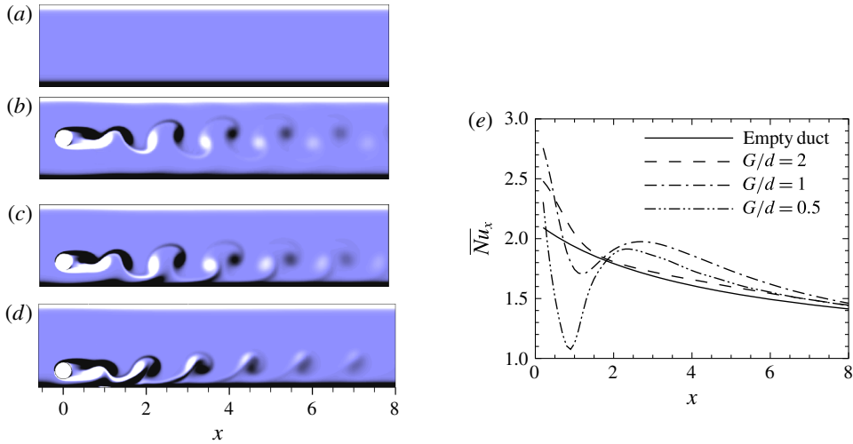
FIGURE 5. (Colour online) (a–d) Instantaneous vorticity contour plots and (e) time-averaged local Nusselt number in the downstream of cylinder. In (a–d), contour levels range between -2 and 2 , with light and dark contours representing positive and negative vorticity, respectively. (a) Shows the case without a cylinder, while (b–d) respectively show cases G/d = 2, 1 and 0.5 .
